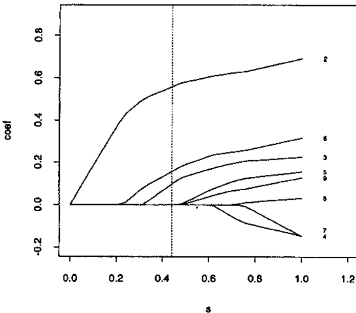
Fig. 5. Lasso shrinkage of coefficients in the prostate cancer example: each curve represents a coefficient (labelled on the right) as a function of the (scaled) lasso parameter s = t/\sum|\hat{\beta}_j^0| (the intercept is not plotted); the broken line represents the model for \hat{s} = 0.44 , selected by generalized cross-validation
